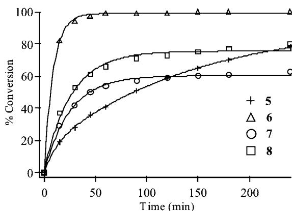
Figure 2. Conversion curve of the ROMP of norbornene using catalysts 5 – 8 (800 equiv. norbornene).
